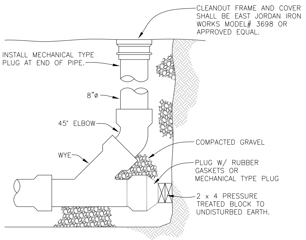
ELEVATION VIEW
